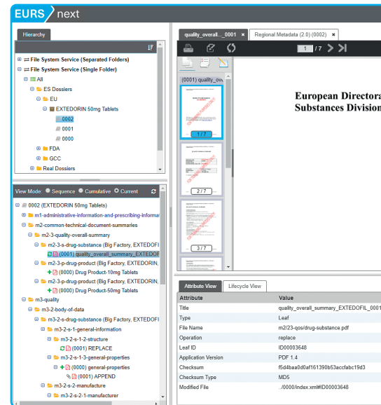
EURSnext: view and review submission data directly within a web browser
